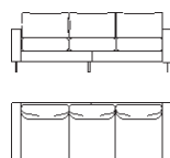
4-zits bank Riverdance W 2530 x D 970 x H 850
