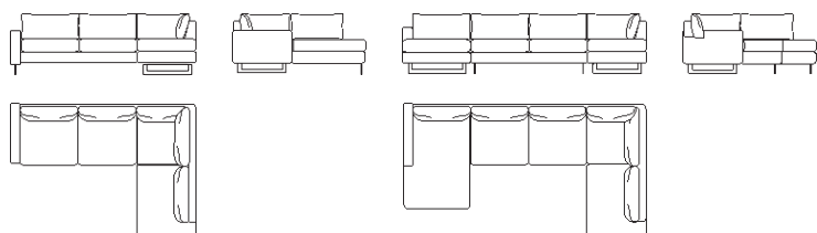
Loungebank Riverdance W 2900 x D 2170 x H 850
